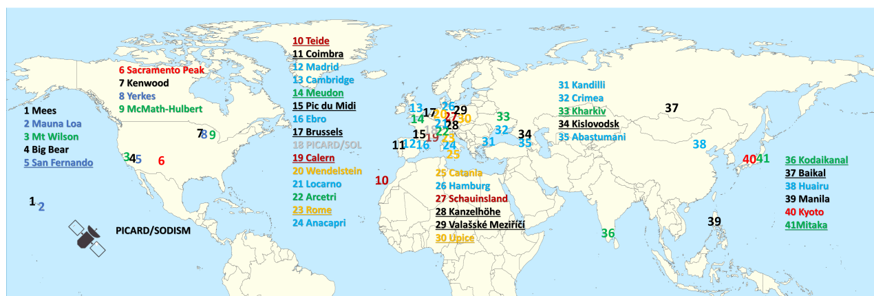
Figure 1. Map showing approximate locations of the Ca II K observatories. Observatories marked in ciel either do not yet have data in digital form or there have been no published results from the digital images. All other archives are shown in various random colours. The locations are marked by numbers, while the names of the sites are listed with the corresponding numbers and colours to help associating the name with the observatory. The underlined names refer to sites performing Ca II K observations at present.
