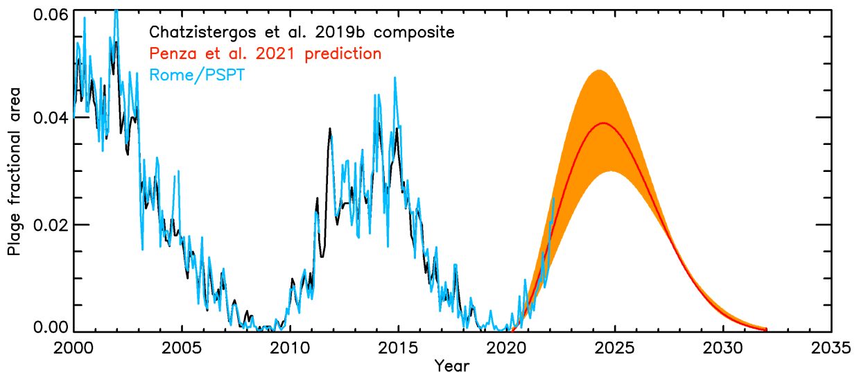
Figure 11. Prediction of solar cycle 25 amplitude in plage fractional areas by Penza et al. (2021, red, with confidence intervals in shaded orange surface). Shown also is the Chatzistergos et al. (2019b) plage area composite (black), on which the prediction was based, as well as more recent data from Rome/PSPT (light blue), which was the reference observatory in the Chatzistergos et al. (2019b) plage area composite since 1996.
